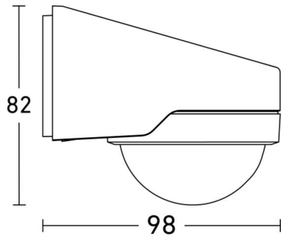
Dimension Drawing 2
